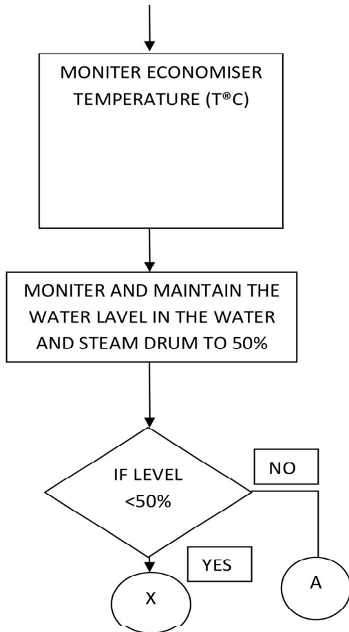
Fig.4, Flow chart of Boiler Operation
