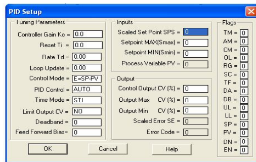
Fig. 3, PID Controller in SCADA
