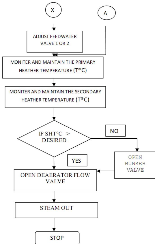
Fig.4, Flow chart of Boiler Operation
