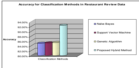
Figure 1: Classification Accuracy of Restaurant Review
