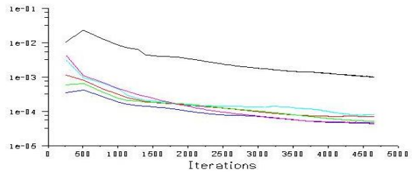
Figure. 12. Residuals for no obstruction plate design. (White-continuity, Red- x.velocity, Green- y.velocity, Blue- z. velocity, Sky Blue- k, Pink- epsilon).
